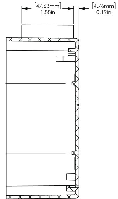
SECTION C-C
