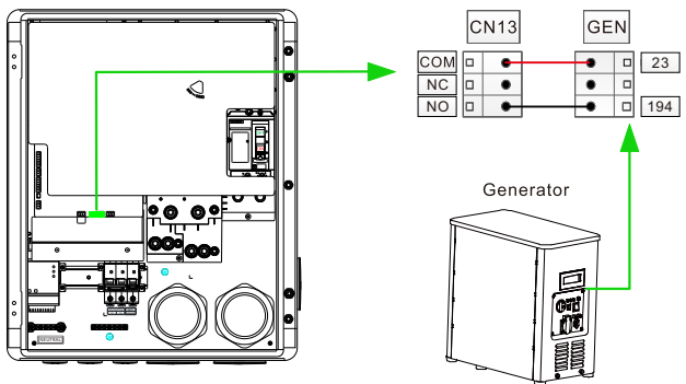
Communication connection between SYN 200-XH-US and Generator
