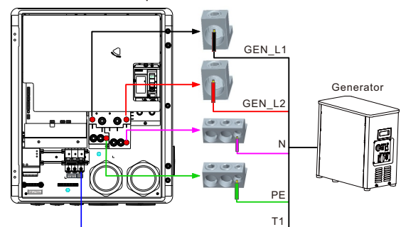
Connection to the Generator
