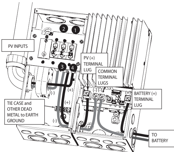
Figure 7. Completing Wiring
