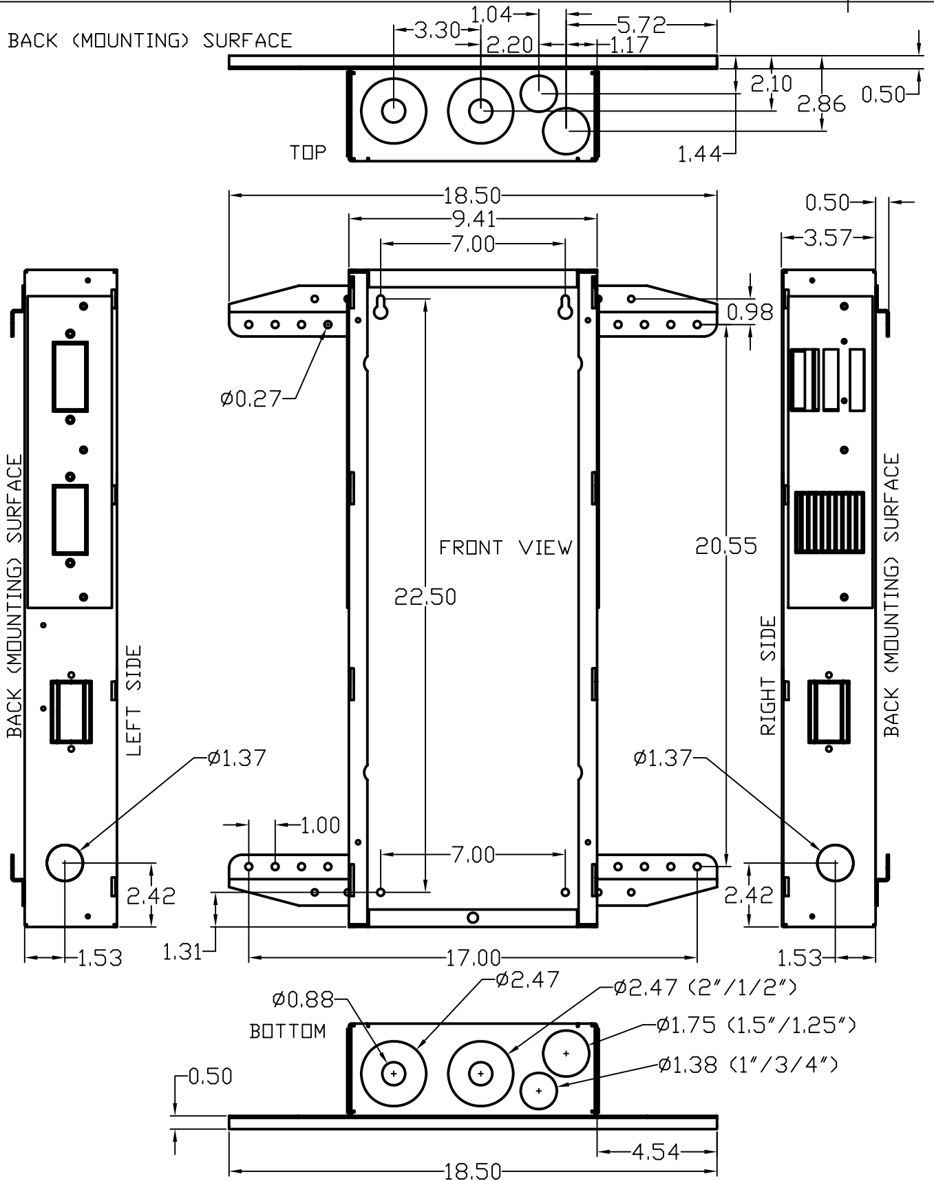
OutBack Configuration
