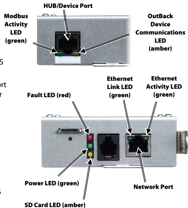
Figure 6 LED Indicators
