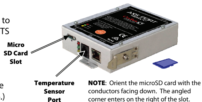
Figure 5 Accessories
