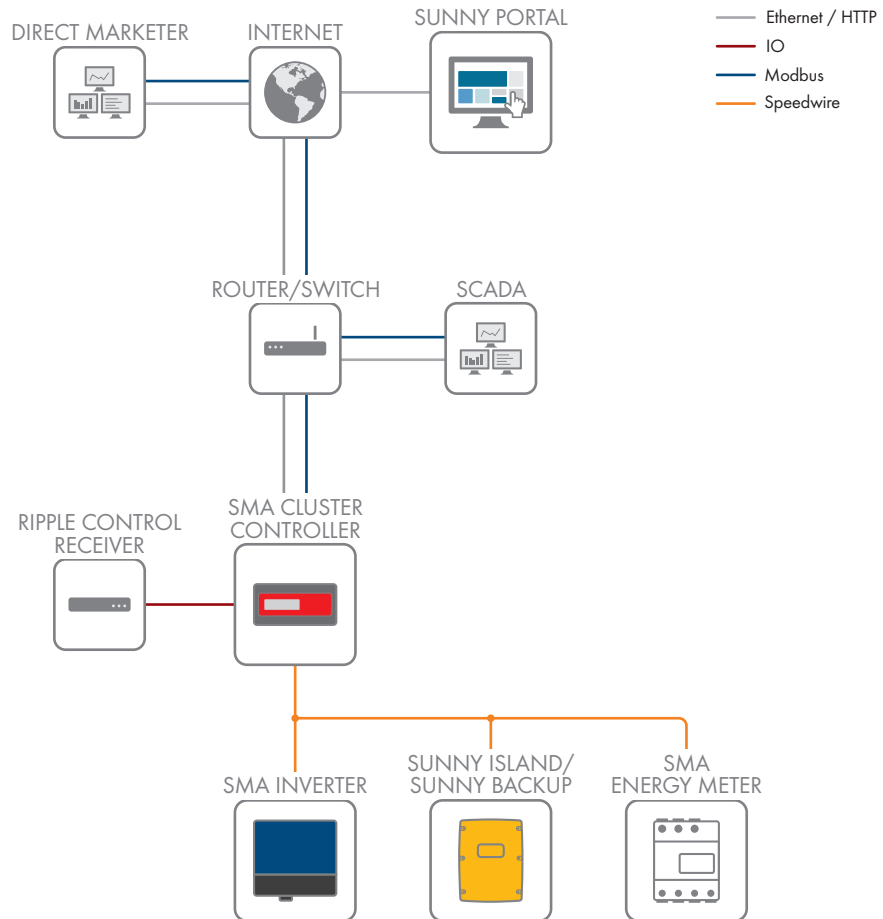
Figure 2: PV system with modern Speedwire communication
