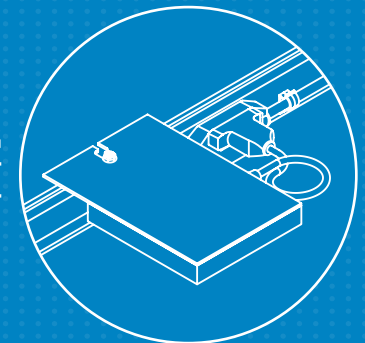
INTEGRATED BONDING MICROINVERTER MOUNT w/ WIRE MANAGEMENT
